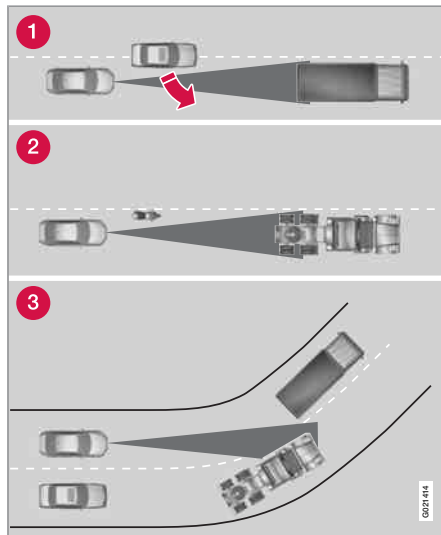
Radar sensor field of vision (gray)
