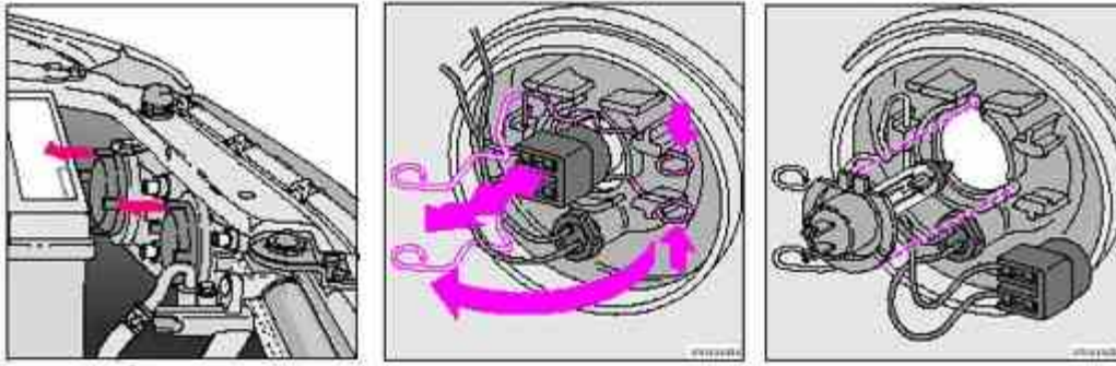
Remove cover
