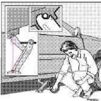
Jack attachment - front wheel drive models
